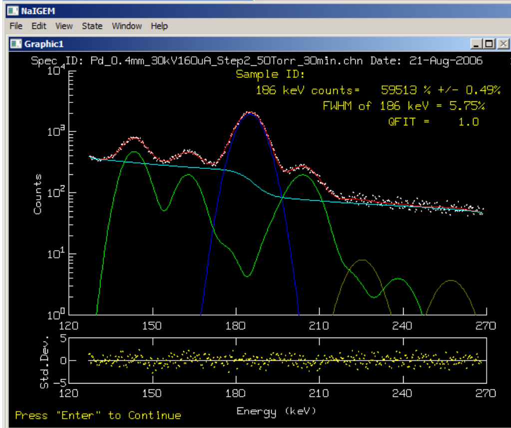
Figure 7-1: Example of a NaIGEM fit used to determine the net area of the 186-keV peak. There is 50 Torr of \text{UF}_6 gas in the pipe, and the measurement was performed on Step 2, the middle (0.5 cm) thickness.
