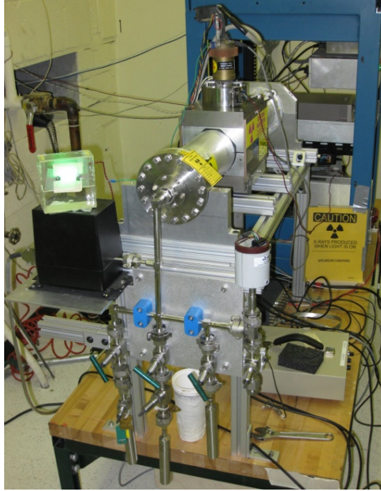
Figure 5-4: Refurbished horizontal source. Shown are the new ½” diameter pipes and the two bottles of UF_6 (foreground, bottom). The bottle on the right is empty.
