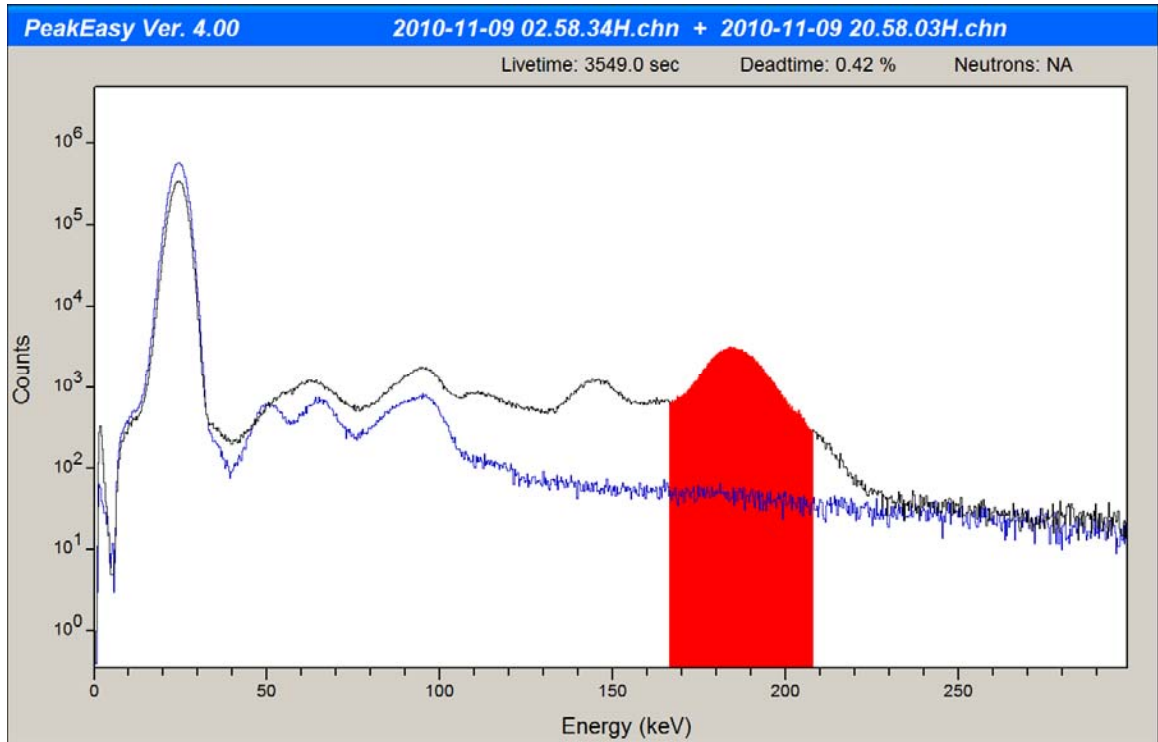
Figure 5-11: Spectra with UF_6 gas (black) and without UF_6 gas (blue) in the pipe. The red coloring shows the ROI for the 186-keV peak.
