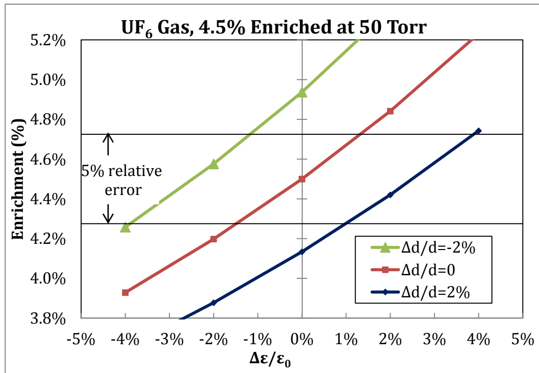
Figure 7-3: Example of enrichment values calculated as described for \text{UF}_6 gas at 4.5% enrichment and 50 Torr pressure. These values were calculated at a transmission energy of 30 keV. The range of instrumentation errors for varying wall thickness error is shown. Specifically detailed is the area that falls within the 5% relative error limit set by mass balance requirements.
