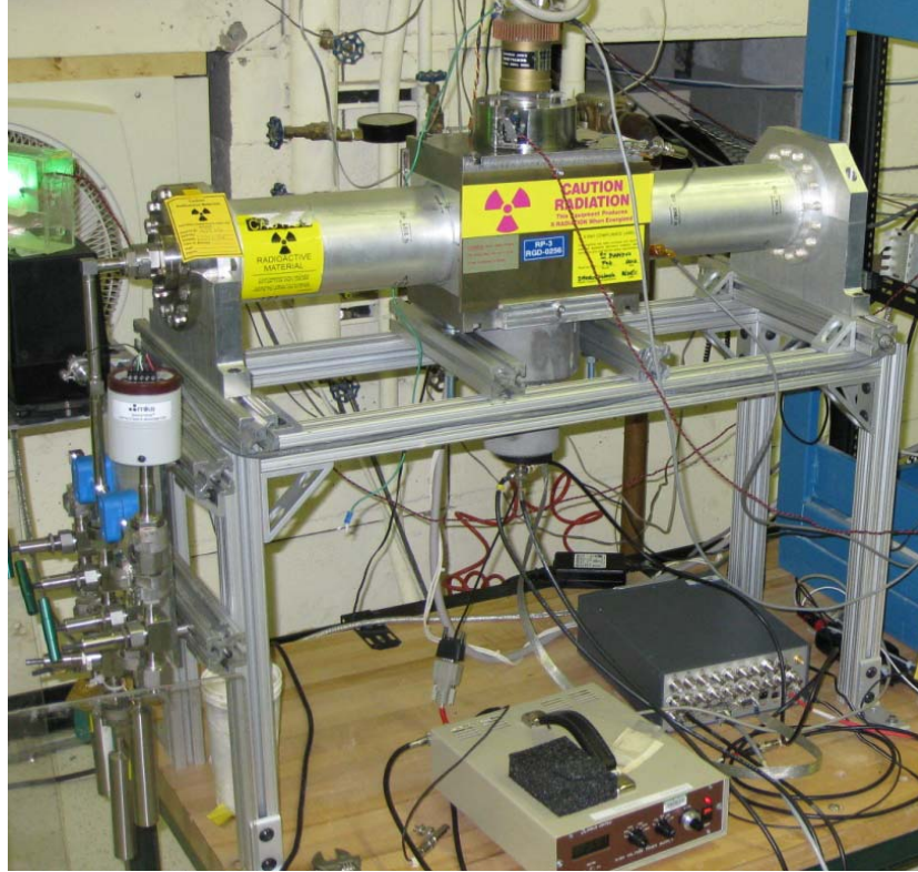
Figure 3-8: Large horizontal UF_6 source with three pipe thicknesses, variable gas pressure, and variable enrichment. The active system is mounted on the pipe with the x-ray tube on the top pointing downwards; the LaBr_3 detector is mounted on the bottom in its tungsten composite shielding.
