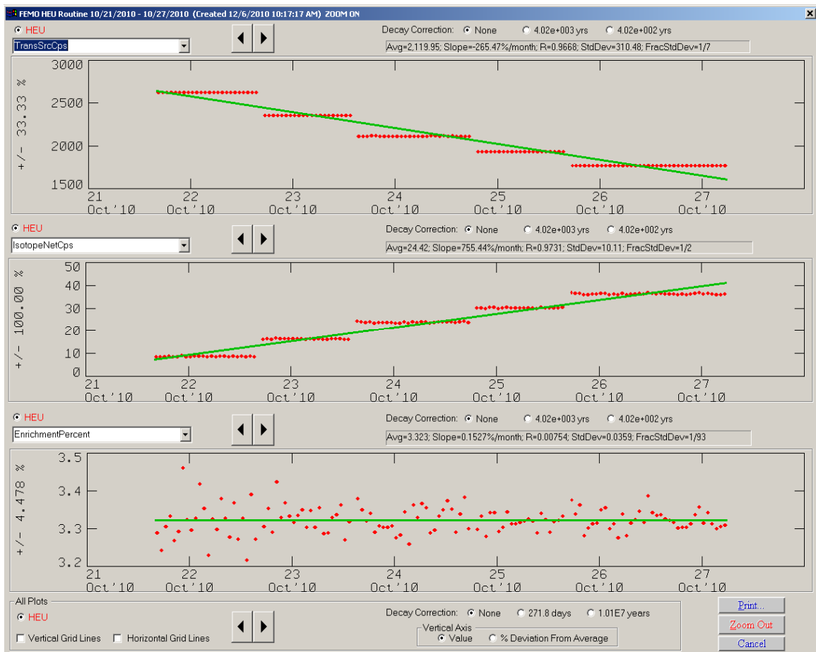
Figure 5-12: Performance of the system with varying pressures of \text{UF}_6 gas. Left to right: 20, 30, 40, 50 and 60 Torr. The top plot shows that the net area of the 25.5-keV silver transmission peak decreases with increasing gas pressure (once background has been subtracted). The middle plot is of the 186-keV peak. The bottom plot shows the calculated enrichment. Red points are individual data points collected when each spectrum was saved, and the green lines are a trend line of the data.
